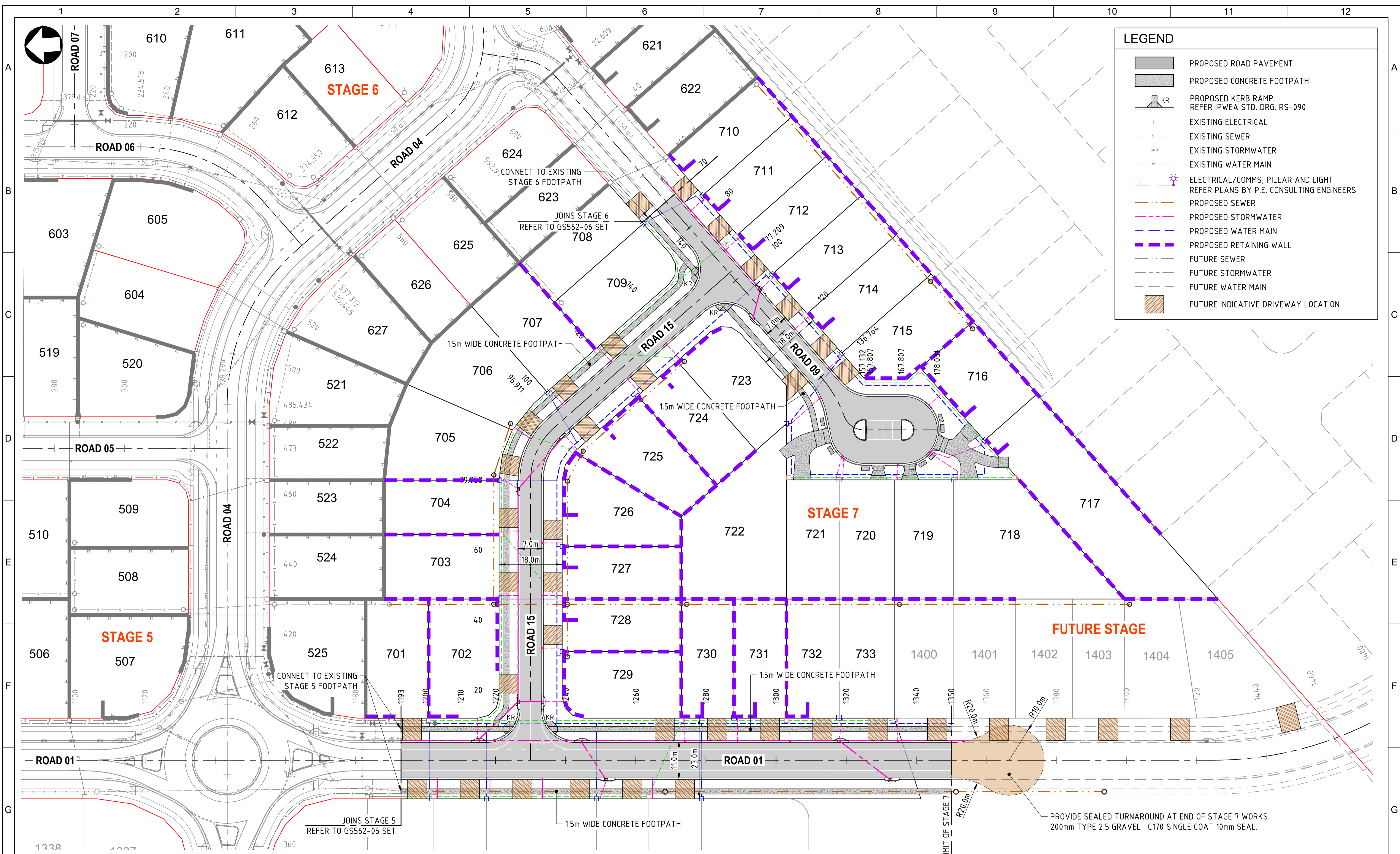
ROADS AND FOOTPATHS LAYOUT PLAN SCALE 1:500
