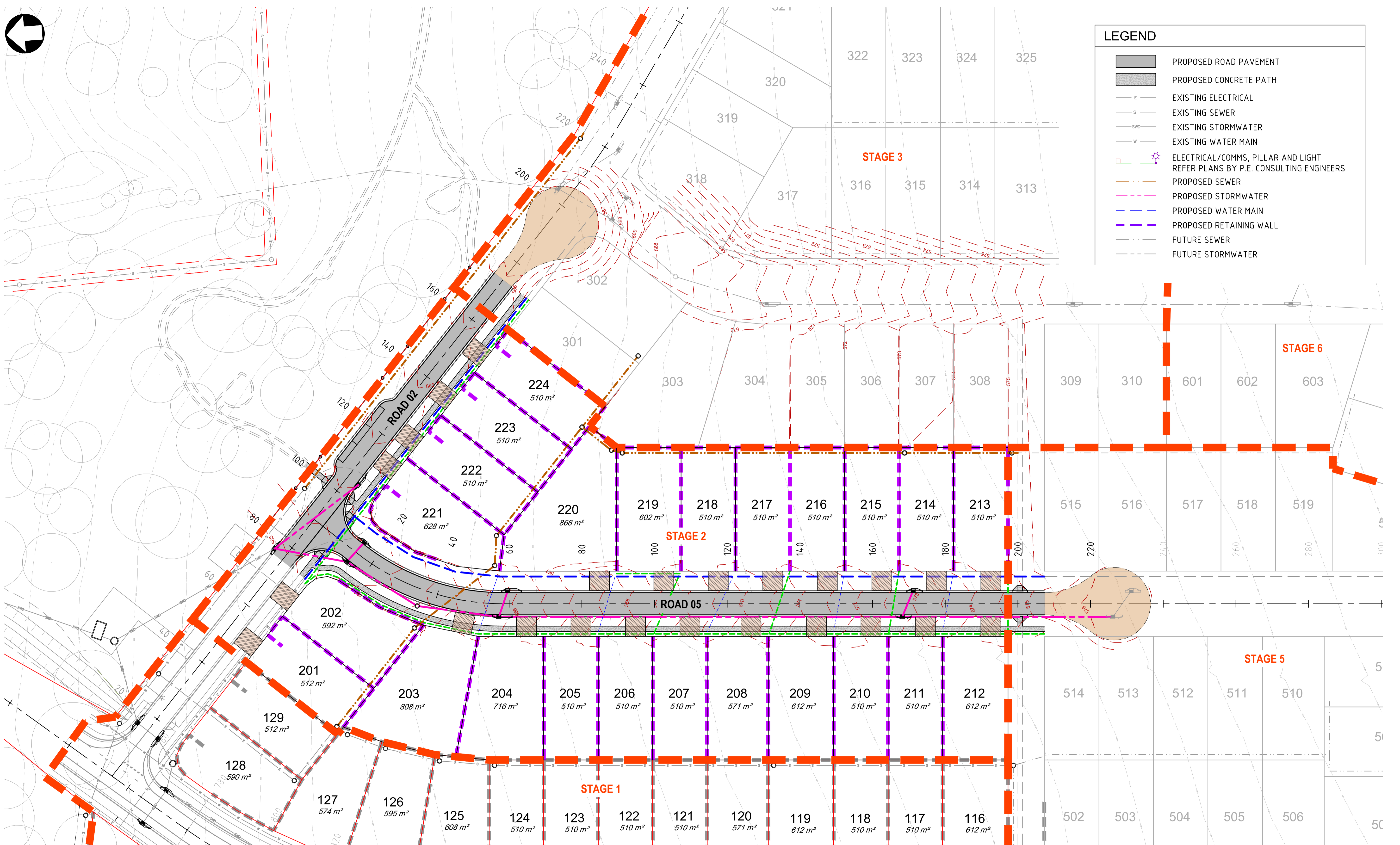
STAGE 2 DEVELOPMENT LAYOUT PLAN
